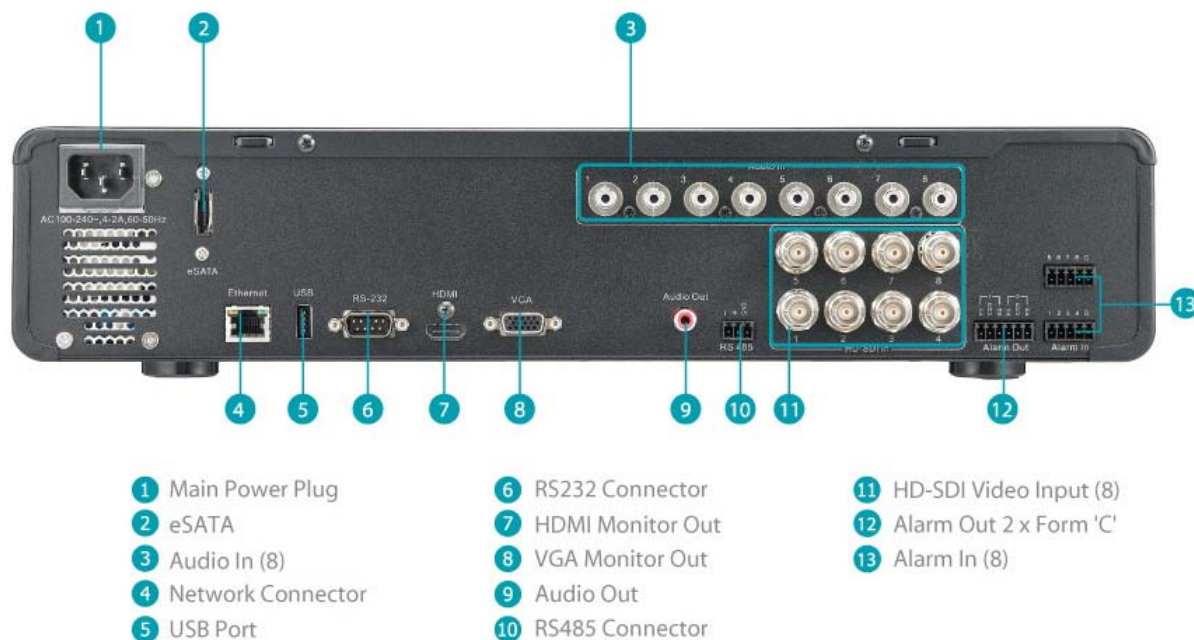
Figure 1-2 Rear Panel
