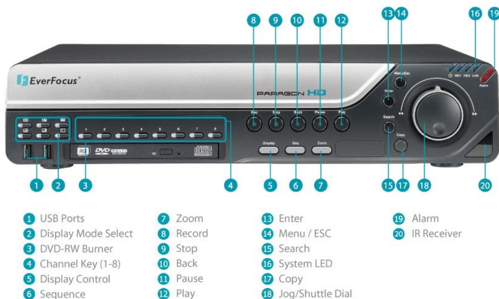
Figure 1-1 Front Panel
